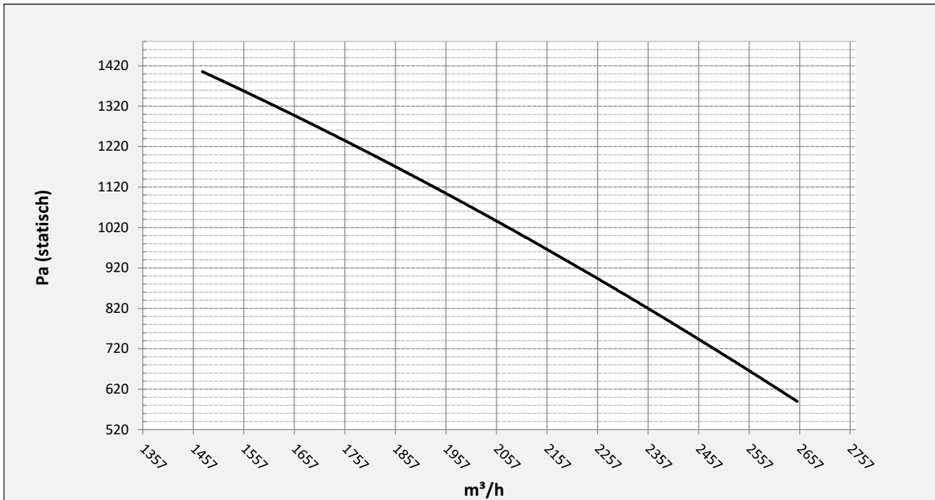
Grafiek EU 311 @ 2830rpm @ 15°C @ 0m
